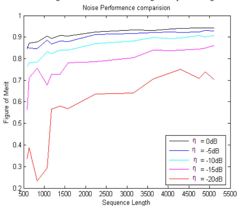
Fig. 2. Noise performance of poly semantic sequences
