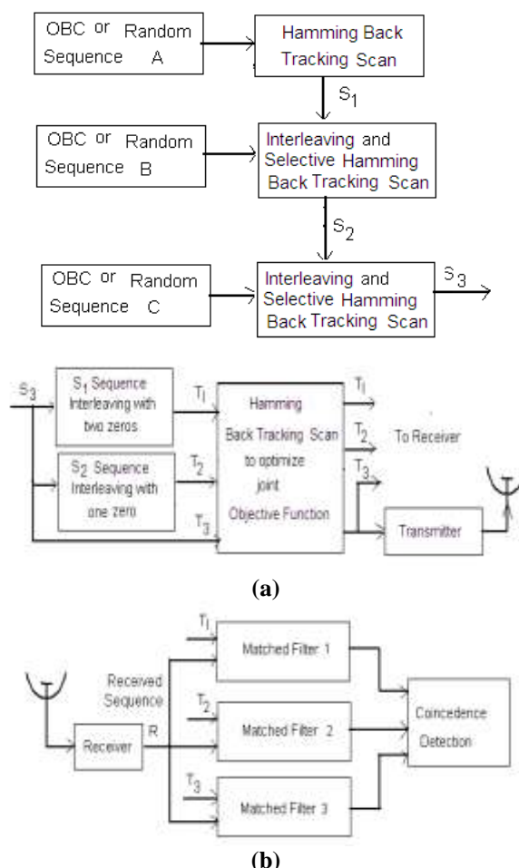
Fig.1. Block schematic diagram of poly-semantic radar signal processor (a) Transmitter (b) Receiver.
